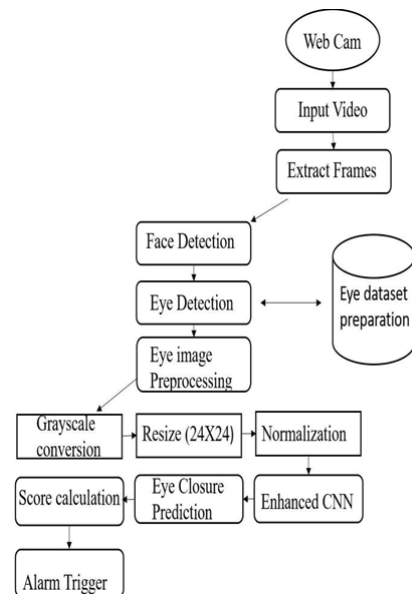
Fig. 1 System Architecture of CNN
