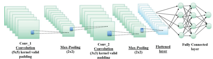
Fig 2. Enhanced CNN Architecture
