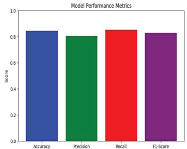
Fig. 5. Performance results of Navie Bayes
