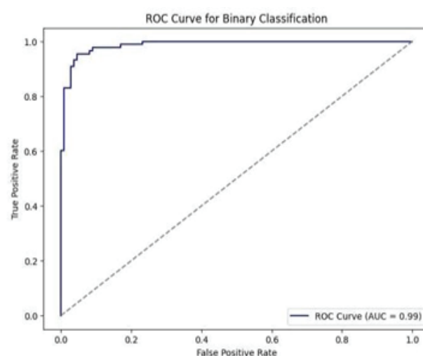
Fig. 2. ROC-AUC Scores of models used
