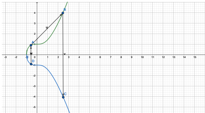
Figure 1: Elliptic Curve
